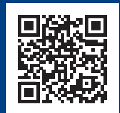
CommandCentral Aware
